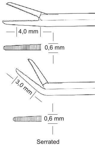
HARTMANN 24-151-14 - 24-154-14 Standard 14 cm / 5 1/2"
